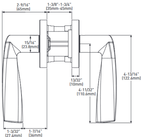
LOQUET 6-EN-1 VERROUILLABLE/NON VERROUILLABLE
